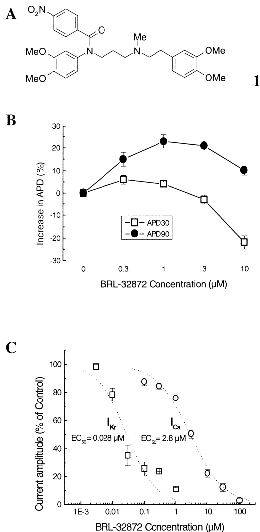
Figure 1. (A) Structure of BRL-32872. (B) Action potential duration recorded on guinea-pig papillary muscle at 30% and 90% of repolarization using standard microelectrode technique. (C) Isolated L-type calcium (circles) and delayed rectifier potassium (squares) currents.
